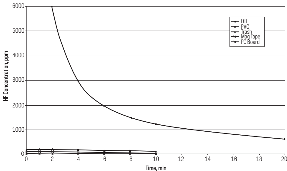
Figure 1. HF Concentrations Relative to Fire Extinguishment with FE-25™
