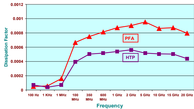
Figure 12. Dissipation Factor of HTP Resin
